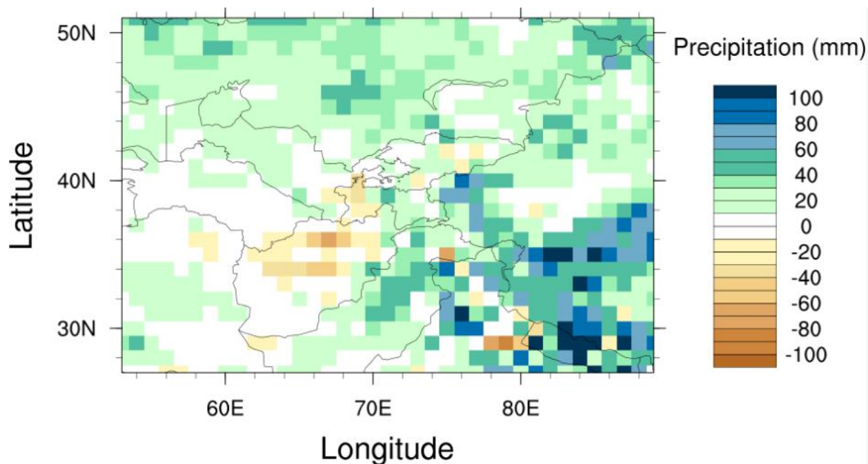
Figure 11: The map shows change in projected Mean Annual Precipitation by 2050 compared to the reference period (1986-2005) under RCP 8.5 of CIMP5 ensemble modeling. Blue/Green areas are likely to receive more annual rainfall compared to the reference period and to Brown/Yellow areas.
