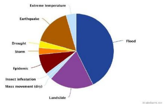
Figure 27: Average Annual Hazard Occurrence for the period 1900-2018
