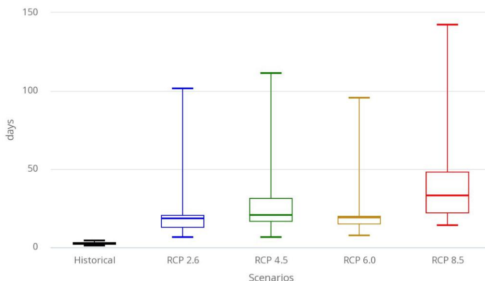
Figure 25: The boxplot shows recorded Warm Spell Duration Index (WSDI) for 1986-2005 and projected WSDI by 2050 under all RCPs of CIMP5 ensemble modeling. The WSDI is a measure of such an uninterrupted sequence of at least 6 days that surpass the currently observed 95th percentile of temperature. It therefore not only reflects increases in temperature but looks at the likelihood of sequences of conditions that today are considered the warmest conditions in the year.
